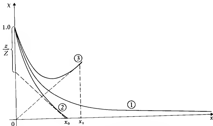
7.4 The three categories of solutions of the Thomas–Fermi equation: (1) neutral atom solution; (2) solution corresponding to a positive ion ( N < Z ); (3) solution corresponding to a neutral atom under pressure.
